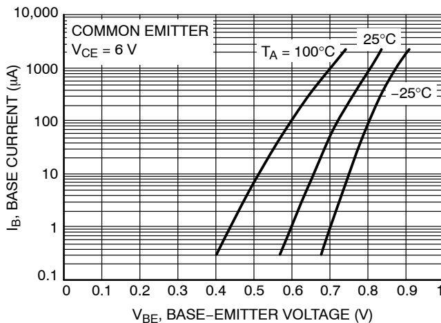
Figure 12. Base-Emitter Voltage
